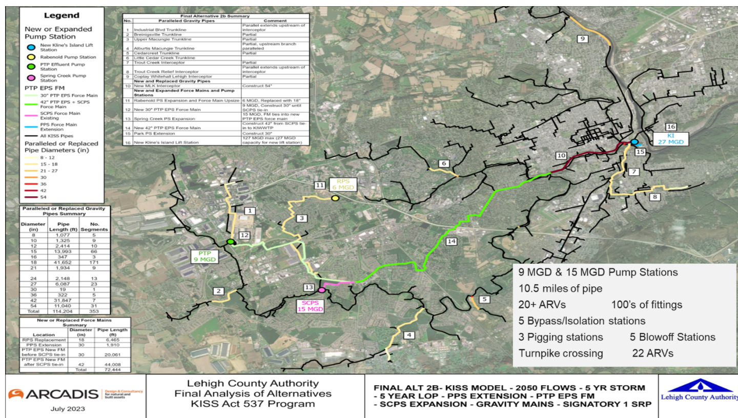
Figure 8 - SOS 2 - PTP EPS and Forcemain
