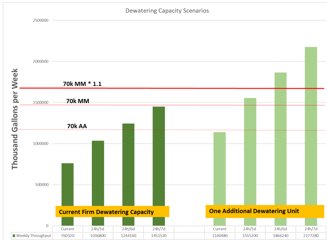
Figure 5 – Dewatering Capacity Analysis
