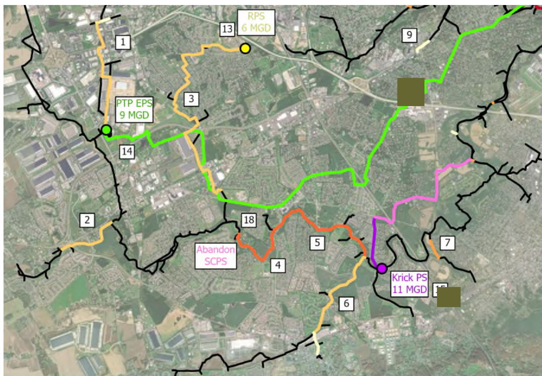
Figure 5 - Krick's Lane Pump Station to eliminate SCPS
