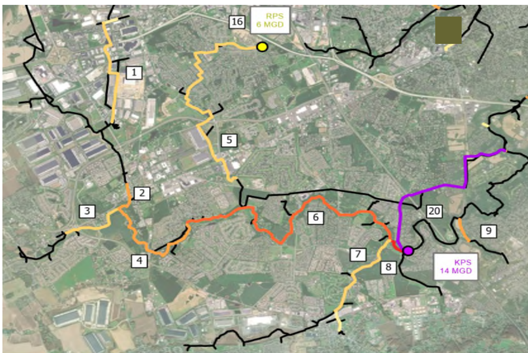
Figure 4 - Krick's Lane Pump Station to eliminate paralleling of Lower WLI
