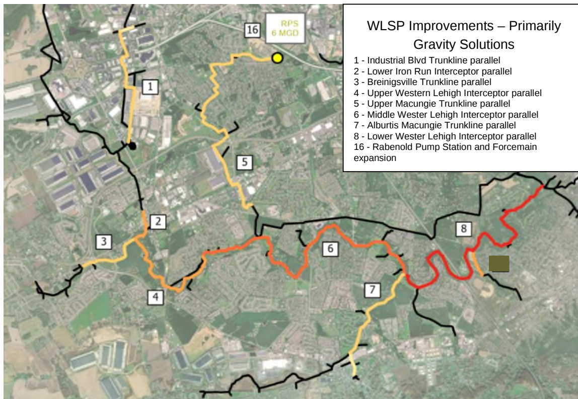
Figure 2 - WLSPI Infrastructure Improvements required to meet Act 537 Goals
