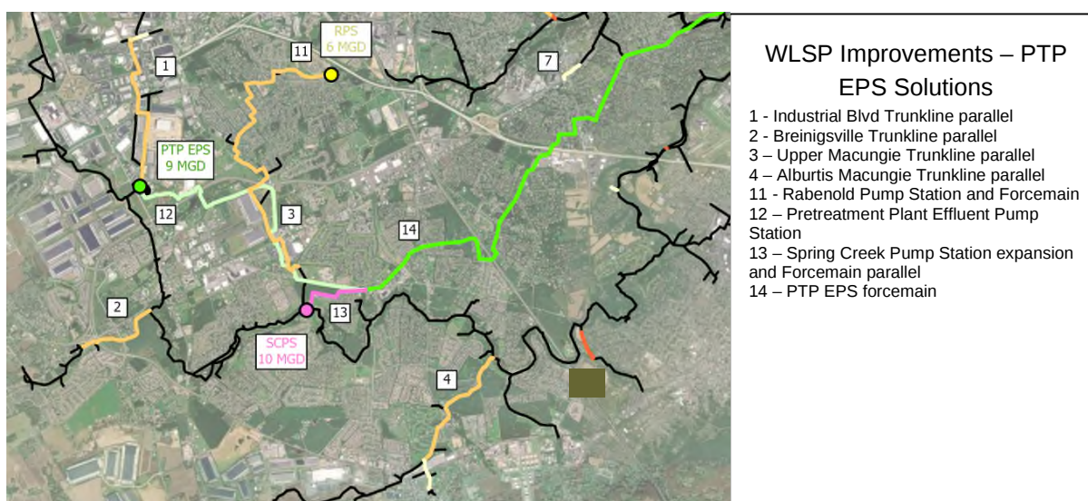
Figure 3 – WLSPI Improvements – Primarily Pumped Solutions
