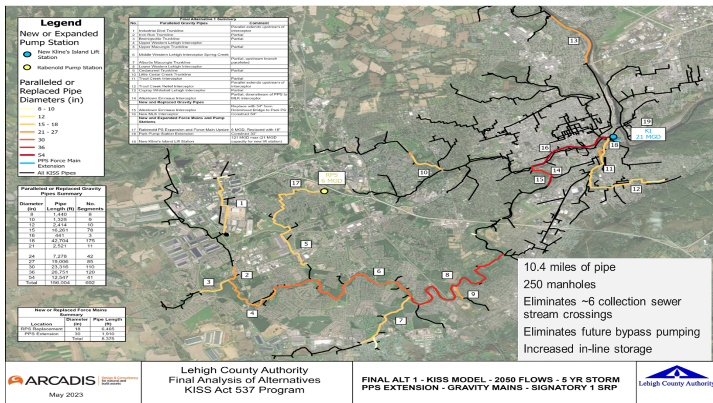
Figure 6 - SOS 1 - Gravity Parallel of WLI
